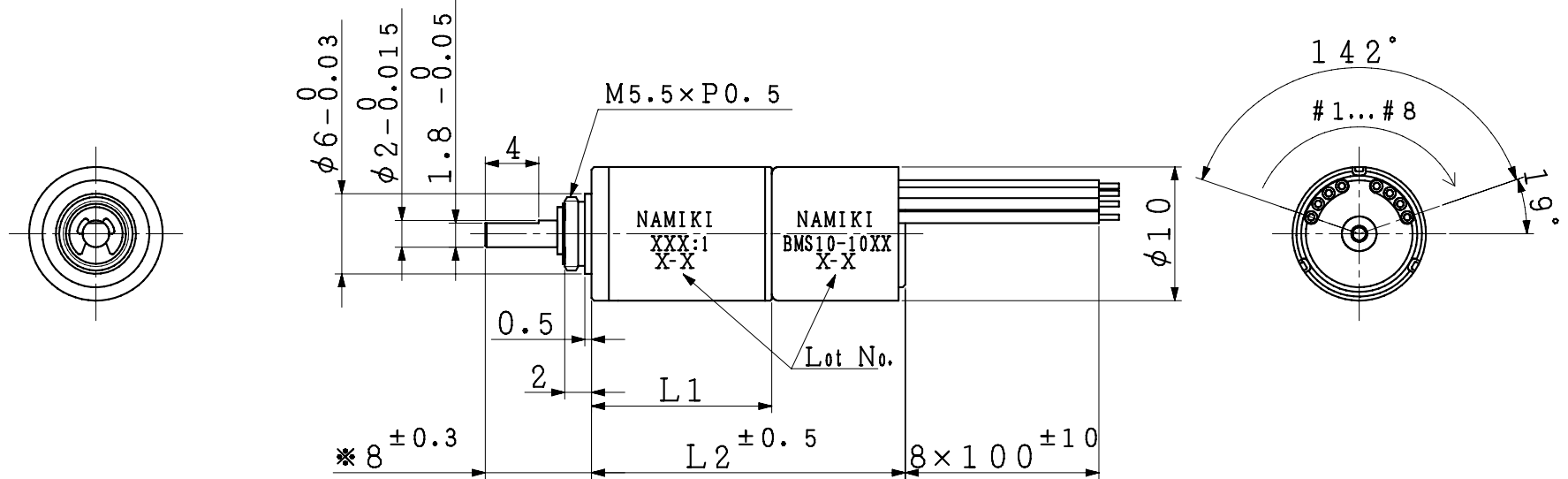
MOTOR LENGTH
