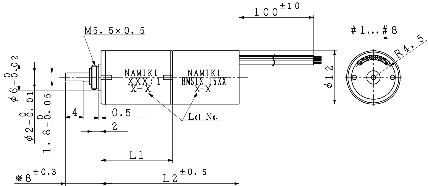
MOTOR LENGTH
