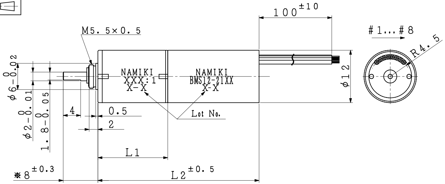
MOTOR LENGTH
