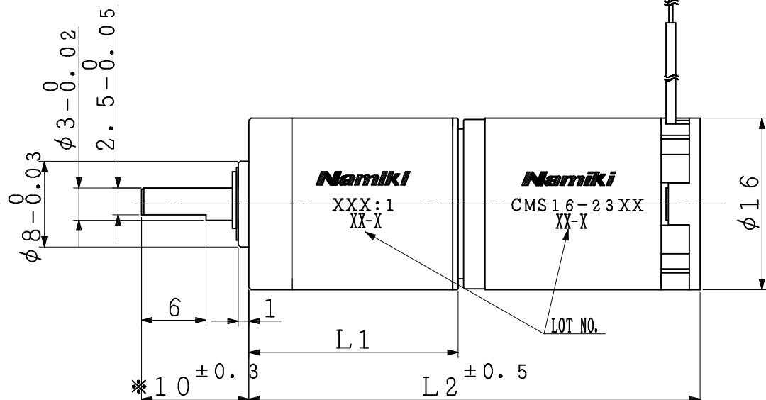
MOTOR LENGTH
